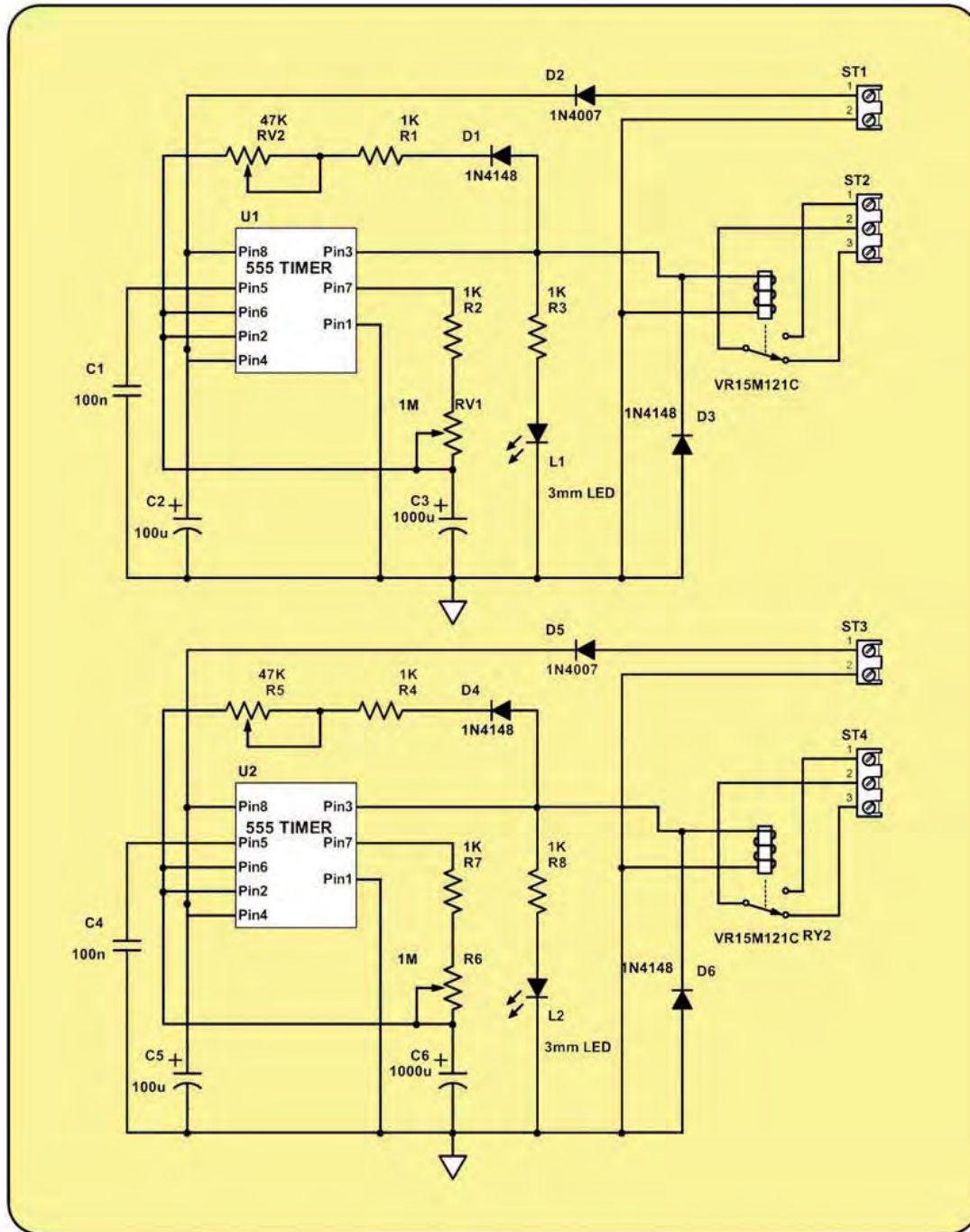
Circuit Board Schematics
